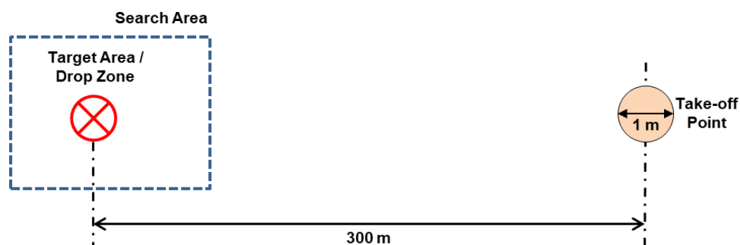
Figure 2 Flight Course
